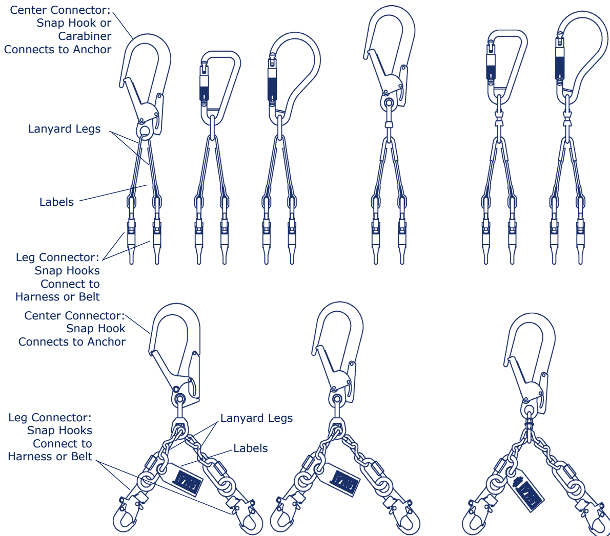
Figure 1 - Rebar Lanyards for Work Positioning
